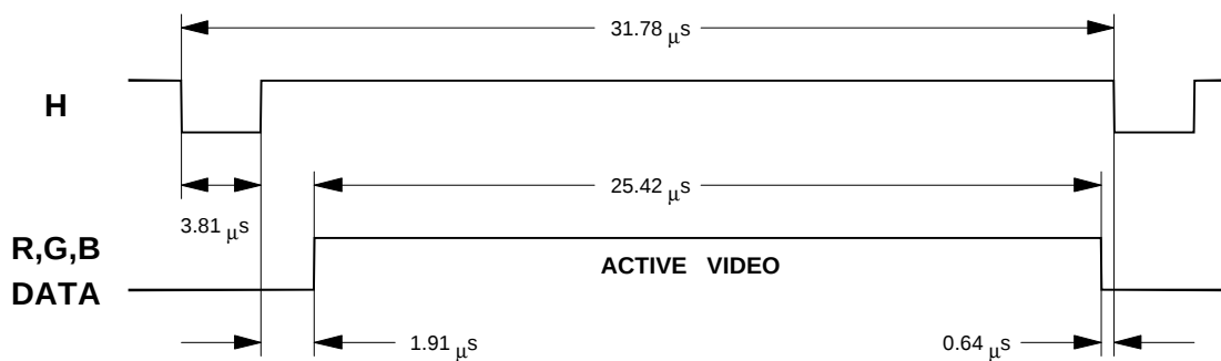
Figure 6: Typical VGA Input Timing
