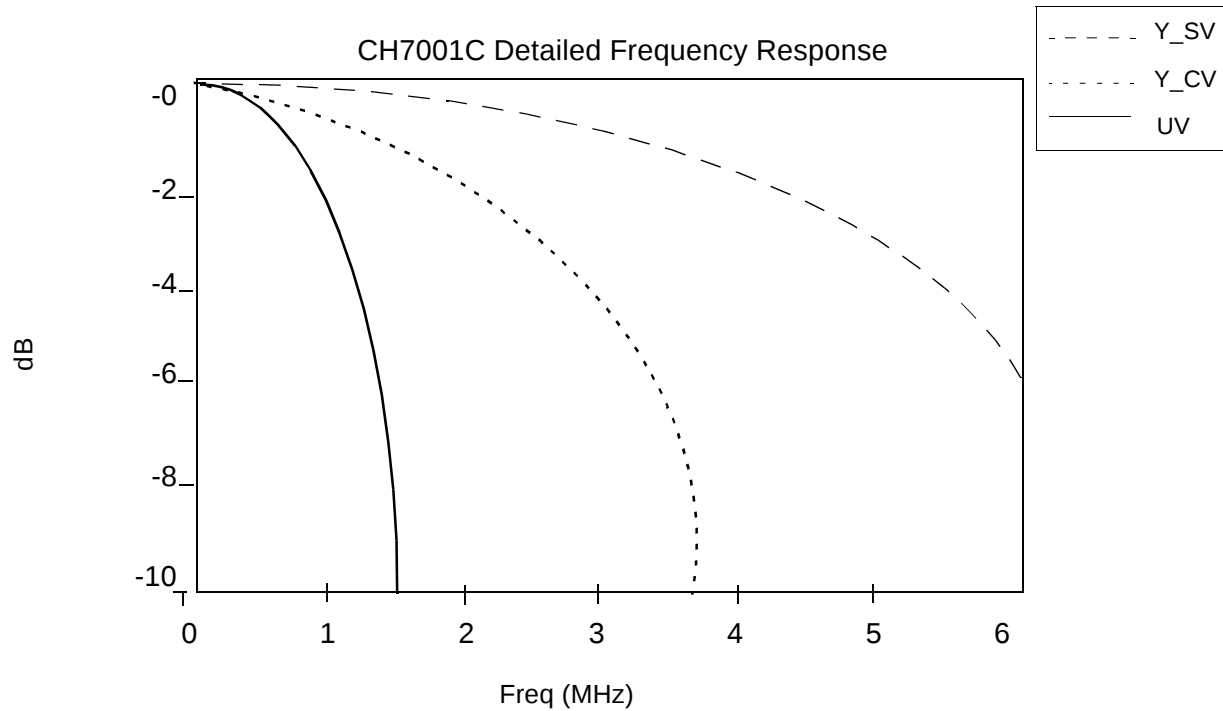
Figure 5: U,V, and Y Filter Response
